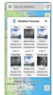
Weather Forecast
