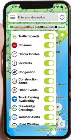
Traffic Speeds
